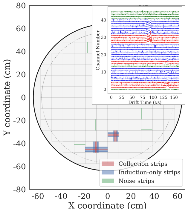
Figure 2. Top view of the charge readout tiles (squares outlined by dotted lines) and current waveform display (inset) showing a multi-site event with energy deposits in three tiles. The red strips and waveforms indicate charge collection, blue strips and waveforms represent induced charge without collection, and the green waveforms only contain noise that triggers the reconstruction algorithm.
