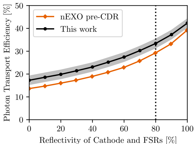
Figure 3. Spatial average PTE inside the fiducial volume as a function of the specular reflectivity of the cathode and the FSRs. The current light simulation results with updated optical parameters (black circles) are compared against results from previous simulations (orange diamonds) [36]. The grey band indicates a systematic error due to the choice of SiPMs and light simulator. The reflectivity value used in the simulations for this work is indicated by the vertical dotted line.
