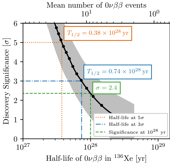
Figure 13. Projections of the median discovery significance to 0\nu\beta\beta decay with 10 years of nEXO data. The grey band indicates the 68% symmetric quantile around the median.
