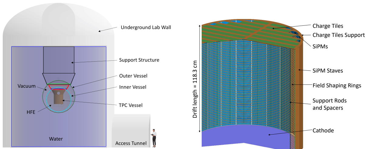
Figure 1. Visualization of the Geant4 geometry implementation for MC simulations of the nEXO detector. The drawing on the left shows a cross-section view of the large components external to the TPC vessel, including the OD’s water and SNOLAB’s Cryopit wall. The model on the right shows a close up view of the main components inside the TPC vessel.
