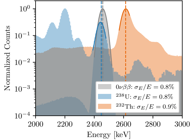
Figure 6. Rotated energy spectra of all simulated events in the FV from 0\nu\beta\beta decays and ^{232}\text{Th} and ^{238}\text{U} decays on the TPC vessel. The vertical lines indicate the expected center of the peaks while the solid lines show their Gaussian fits. The resolutions are calculated by the fitted \sigma_E/E . The three spectra are normalized to have the same maximum value.
