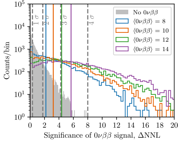
Figure A2. Sample distributions of q_0 for the null hypothesis H_0 in grey and for alternative hypotheses H_\mu in color, with \mu = 8, 10, 12 and 14 . In total 1 \times 10^5 and 5 \times 10^3 toy datasets were simulated for the null hypothesis and the alternative hypotheses, respectively. The p -value is calculated from counting the number of toy datasets in the distribution for H_0 that are above the median value for H_\mu , shown as vertical colored lines. The grey vertical dashed lines indicate the quantiles corresponding to 1\sigma , 2\sigma , 3\sigma and 4\sigma significance of discovery.
