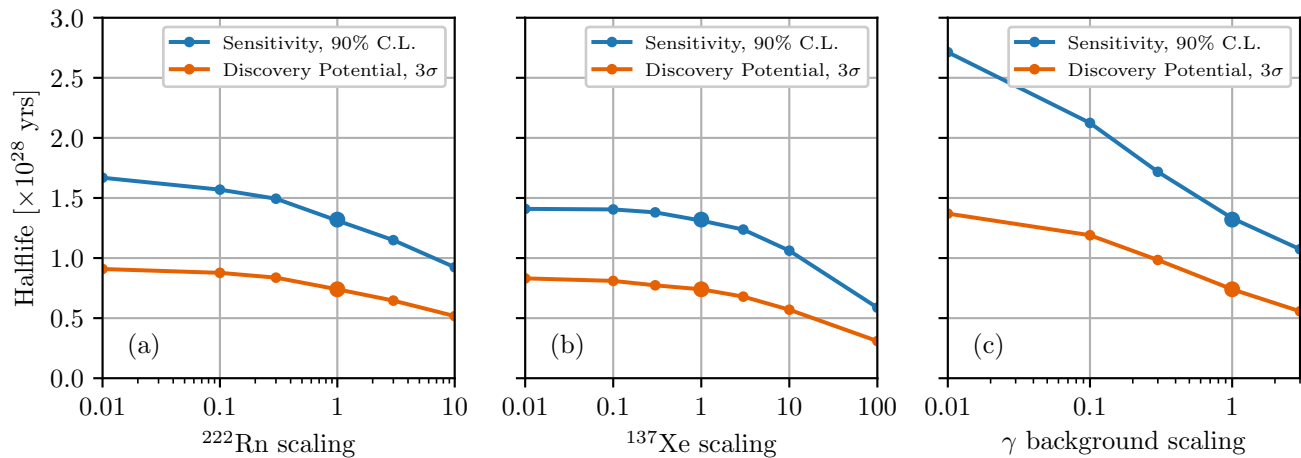
Figure 15. nEXO median sensitivity and 3\sigma discovery potential evaluated for hypothetical variations in background scale from (a) ^{222}\text{Rn} decays in the LXe, (b) ^{137}\text{Xe} production, and (c) all \gamma background components.
