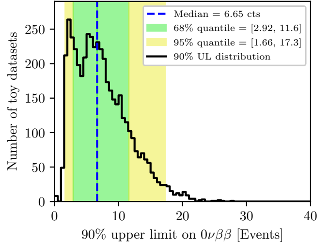
Figure A1. Distribution of upper limits \mu_{90} for 5000 toy datasets. The median corresponds to a bound on the 0\nu\beta\beta decay half-life of T_{1/2} > 1.35 \times 10^{28} years.
