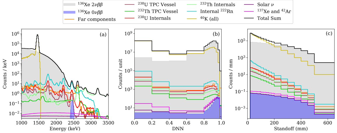
Figure 10. Nominal model of event distributions in nEXO, projected onto each of the three axes used in the sensitivity analysis: (a) event energy, (b) DNN 0\nu\beta\beta discriminator, and (c) standoff distance. The 0\nu\beta\beta decay signal corresponds to a half-life of 0.74 \times 10^{28} yr.
